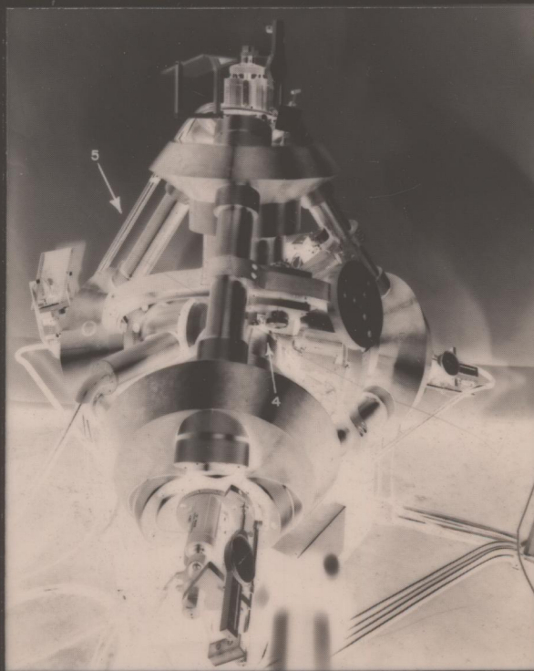
FIG. 2 TETRAHEDRAL-ANVIL PRESS (VIEW 1)
