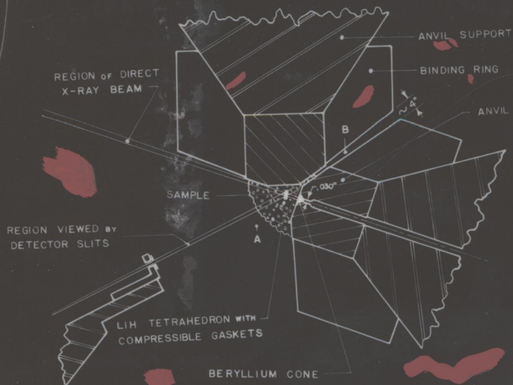
FIG. 8 SAMPLE CHAMBER DETAIL
